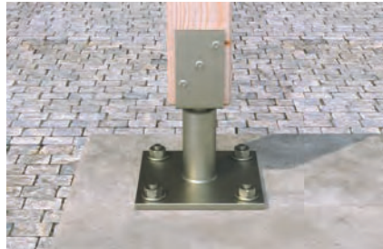
Column bases
